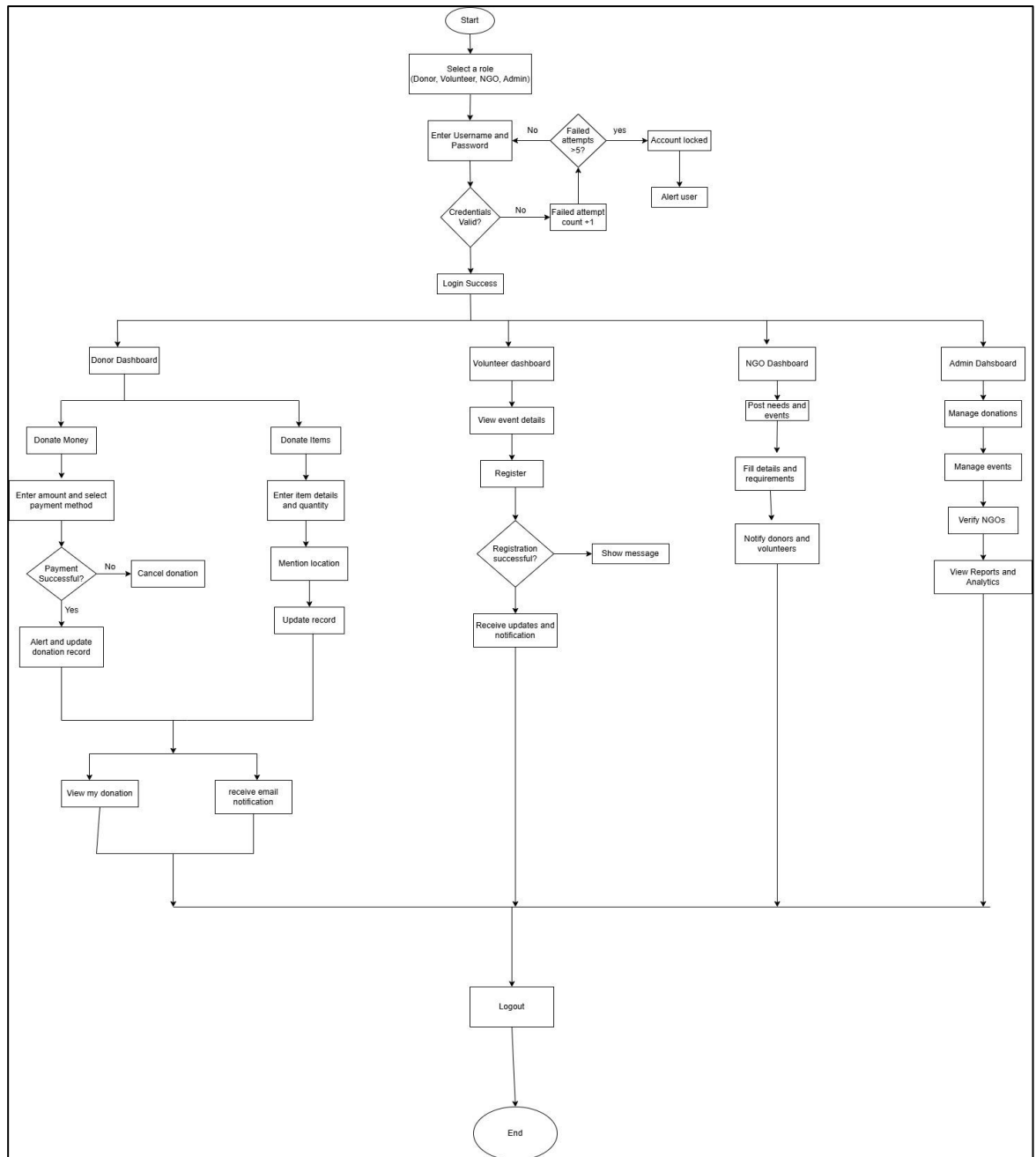
Figure (ii): Flowchart
