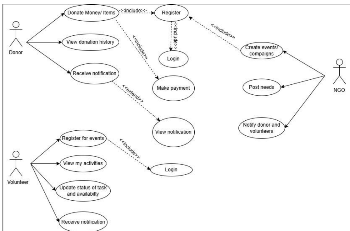
Figure (i): Use Case
